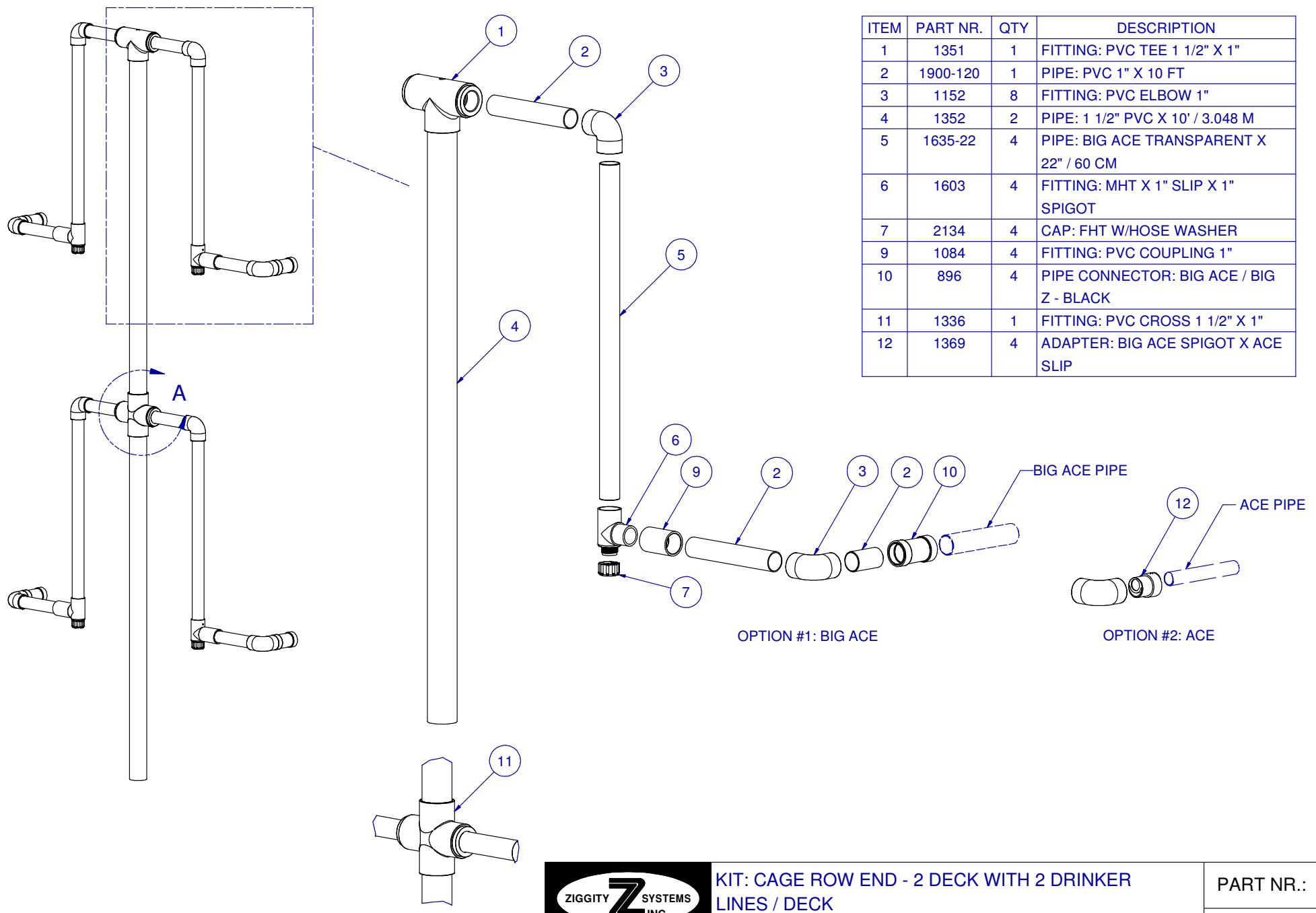
DETAIL A
