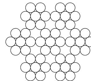
7 X 7 STRAND
