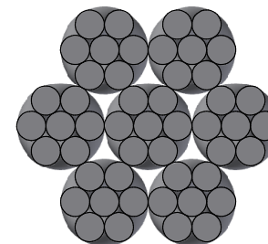
7 X 7 STRAND
